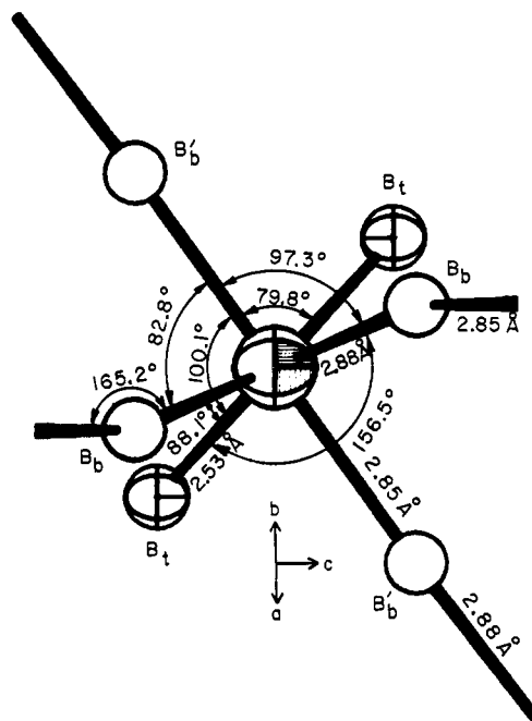
Figure 2. Site symmetry of \text{U}(\text{BH}_4)_4 viewed down the crystallographically imposed C_2 axis. Standard deviations in \text{U}-\text{B} bonds are \pm 0.03 \text{ \AA} , in \text{B}-\text{U}-\text{B} angles, \pm 0.8^\circ , and in the \text{U}-\text{B}-\text{U} angle, \pm 1.0^\circ . Angles not shown are \text{B}_t-\text{U}-\text{B}_t , 110.4^\circ , \text{B}_b'-\text{U}-\text{B}_b' , 179.8^\circ and \text{B}_b'-\text{U}-\text{B}_b , 78.7^\circ .
