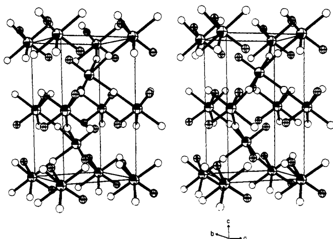
Figure 1. Stereoscopic unit cell packing diagram for \text{U}(\text{BH}_4)_4 . Fourfold screw axes parallel to c intersect the ab plane at (\frac{1}{2}, 0) and (0, \frac{1}{2}) . Lines connecting the uranium (large spheres) and boron atoms are drawn to illustrate the \text{U}-\text{BH}_4 connectivity and are not meant to imply direct \text{U}-\text{B} bonding.
